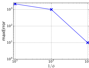
Figure 11: Relation between \phi and maxError. How maxError changes with the change of \phi from 10^{-1} to 10^{-3} .
