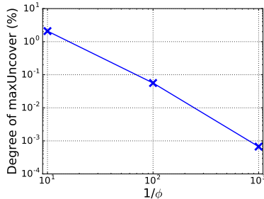
Figure 10: Relation between \phi and degree of maxUncover. How the degree of maxUncover changes with the change of \phi from 10^{-1} to 10^{-3} .
