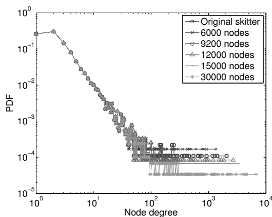
Figure 6: Degree distribution for 1K -rescaled skitter AS topologies
