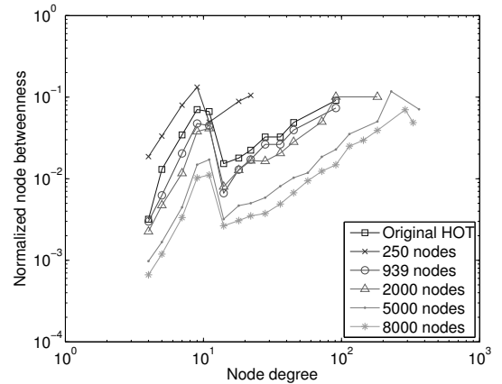
Figure 11: Betweenness distribution 2K-rescaled HOT topologies
