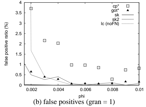
Figure 17: Accuracy without compression
