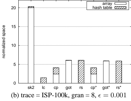
Figure 15: Normalized space costs of different algorithms. (normalized space cost = total space cost / [1/\epsilon \cdot (32/\text{gran})^2] ). The cost for sk (not shown) is 5.5 times more than that for sk2.
