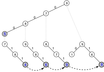
Figure 8: The grid-of-trie data structure after the update operation. The nodes to which we add the size of the current packet are shown in grey. The internal nodes are in light grey. The dashed lines represent jump pointers (which are always between nodes with the same source prefix).
