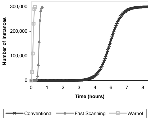
Figure 7: The spread of three simulated worms in a population of 300,000 vulnerable machines: (i) a Code Red-like worm capable of 10 scans/second, (ii) a faster scanning worm capable of 100 scans/second, and (iii) a Warhol worm, capable of 100 scans/second, using a 10,000 entry hit-list and permutation scanning which gives up when 2 infected machines are discovered without finding a new target. All graphs stop at 99.99% infection of the simulated address space.
