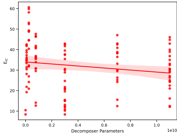
Figure 7: Error induction rate E_{IC} on all datasets (except Winoground) with respect to the number of parameters in the decomposer. There is statistically significant correlation between the number of parameters R^2 = 0.35 . The slope is -0.07 when the unit scale is set to 100M parameters, corresponding to a \approx .7\% increase in E_{CR} for every 1B increase in parameters.
