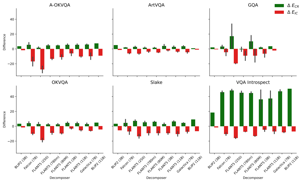
Figure 9: The change in E_{IC} and E_{CR} after selectively decomposing questions.
