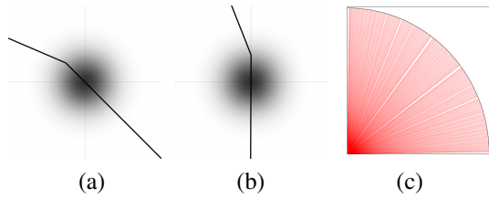
Figure 2: (a) Running example \varphi_{\text{ex}} . (b) Transformed \varphi_{\text{ex}} : T_q\varphi_{\text{ex}} . (c) 2,122 rational unit vectors can be constructed in the first quadrant, using integers with \leq 4 digits.
