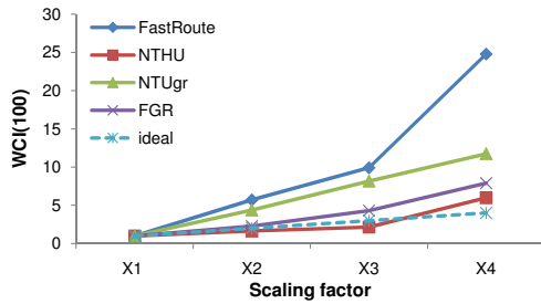
(c) Normalized WCI(100) variation
