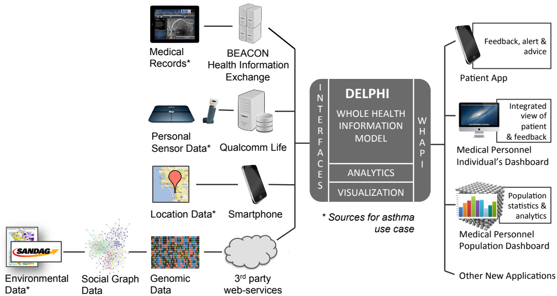
Figure 1. DELPHI Architecture
