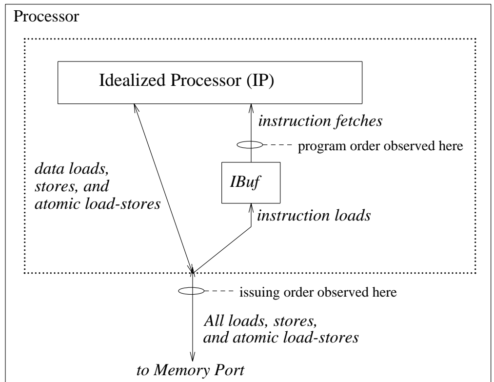
Figure 6-2 Model of a Processor
