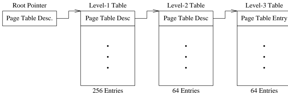
Figure H-3 Reference MMU three-level mapping
