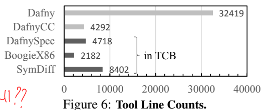
Figure 6: Tool Line Counts.
