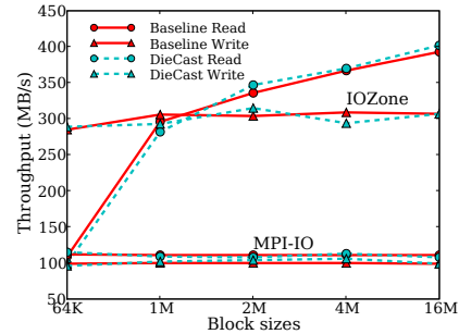
Figure 14: Validating DieCast on PanFS.
