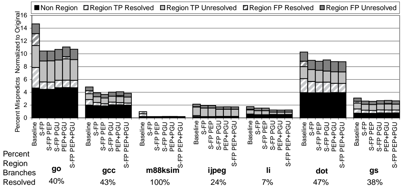
Figure 8: Change in misprediction rate, normalized to the number of predictor accesses in the original unpredicated code. Columns 1 and 5 of each group are not optimized with Squash-FP, the rest show the benefit gained by removing resolved false path predictions. The percent of region branches whose guarding predicate is resolved by branch fetch is shown below each benchmark. PGU can still improve prediction rate when few branch guarding predicates are resolved.
