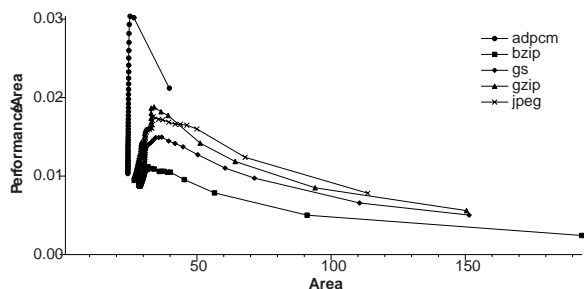
Figure 17: Performance per unit area of the different benchmarks shown as function of total chip area. While performance per unit area may not be useful to an embedded designer, seeking to meet some performance constraint, it is a result that could be easily used by chip multiprocessor designers to help maximize to total processing power of a given chip real-estate.
