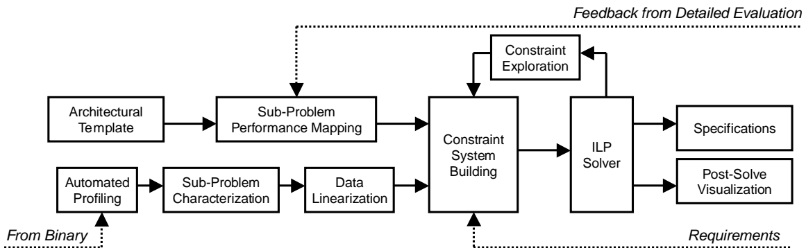
Figure 2: Overview of the Sherpa design guide implementation. The system starts with the input binary and the set of requirements. The binary is profiled and the different sub-problems are analyzed. In the data linearization stage a set of piecewise linear functions are built for each sub-problem. These, along with an automatically constructed performance model, are converted into a constraint system which is solved using integer-linear programming. A set of different constraints can then be iterated over. The output of the solver can then be visualized for human examination and converted into a set of processor specifications for use by synthesis.
