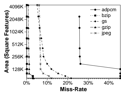
Figure 11: Branch misprediction rate versus area tradeoff. Several branch prediction architectures were examined and the Pareto optimal area/miss rate points are plotted for each program.
