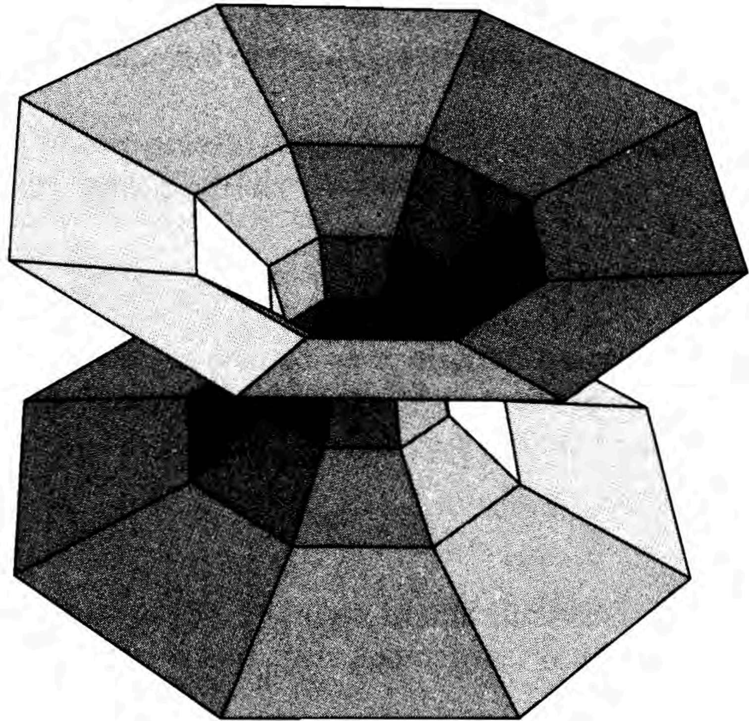
Figure 10. Discrete catenoid
