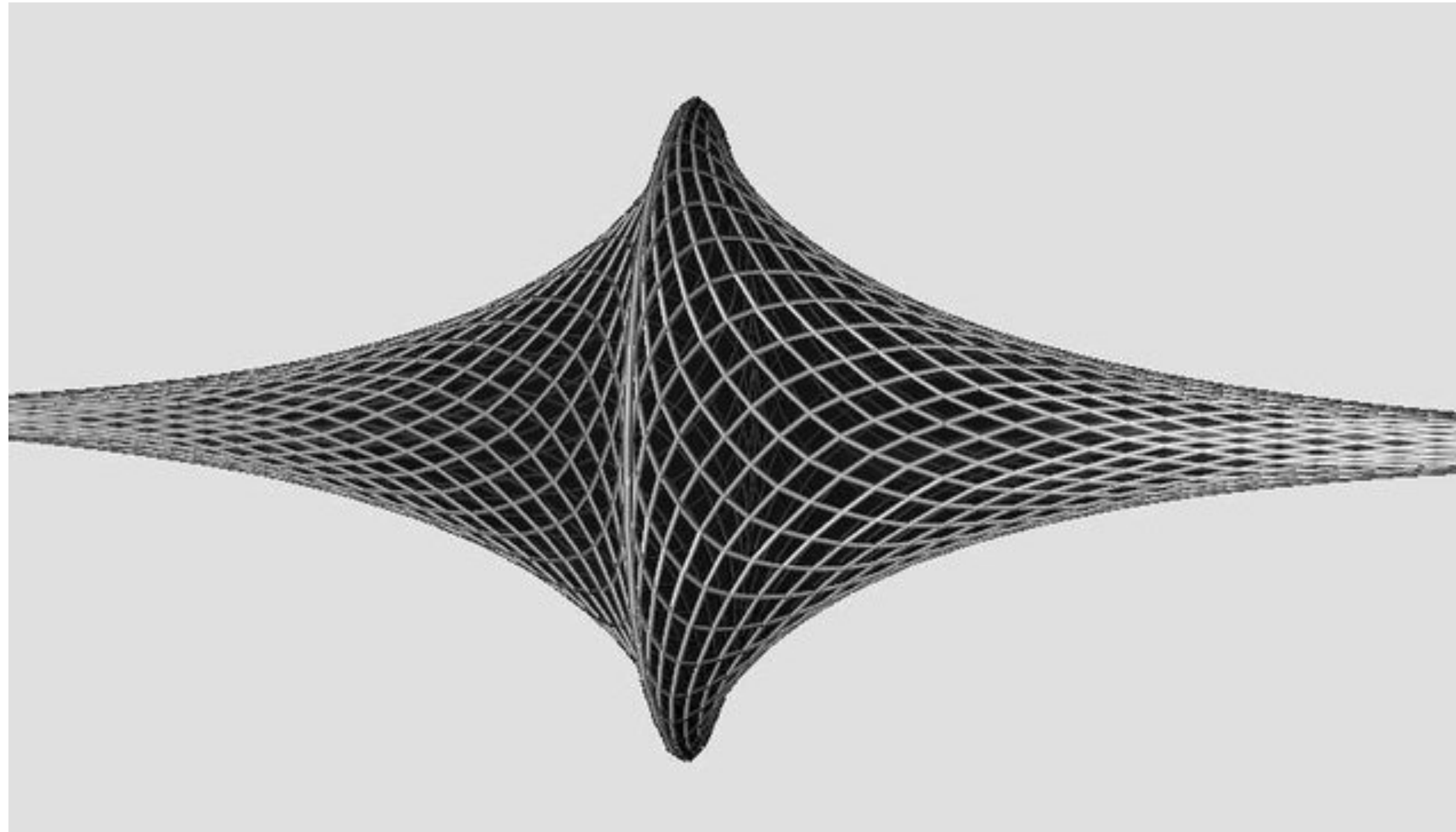
Constant (negative) Gauss curvature surface
