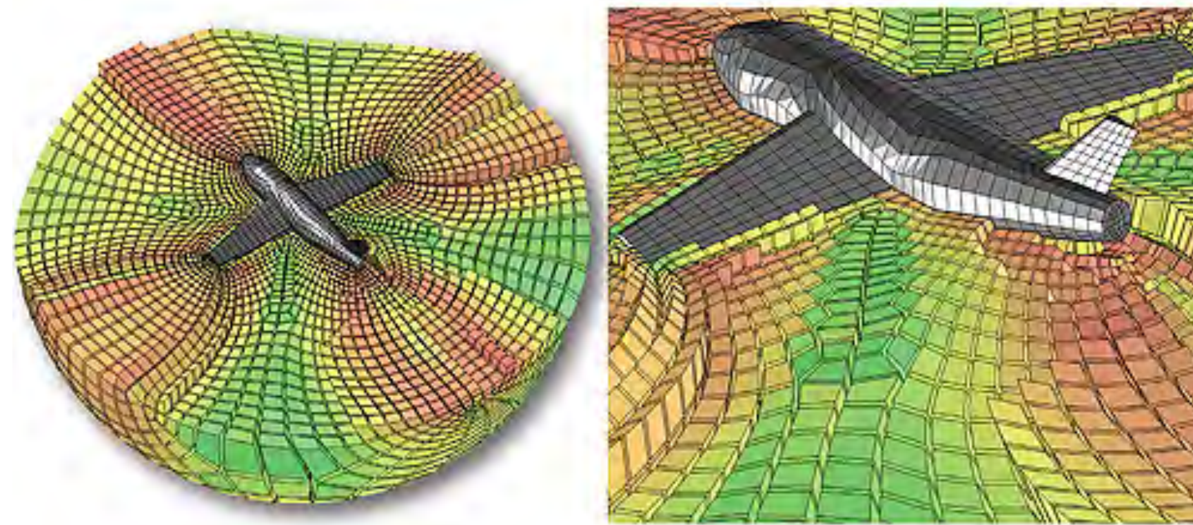
Simulation domain
