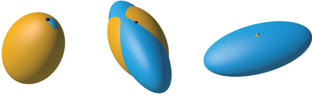
Figure 2 The polhode when the initial angular velocity is close to the axis of (left) smallest \mu , (middle) intermediate \mu and (right) largest \mu , where \mu 's are diagonal values for the diagonal matrix of the moment of inertia \mathbf{M}_{\text{model}} .
