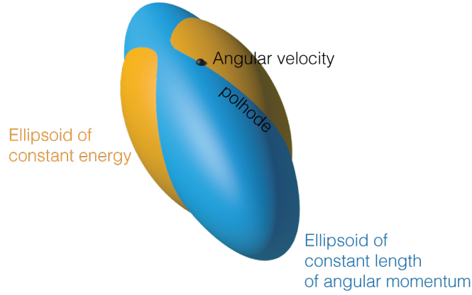
Figure 1 The angular velocity follows the polhode, the intersection of two ellipsoids.
