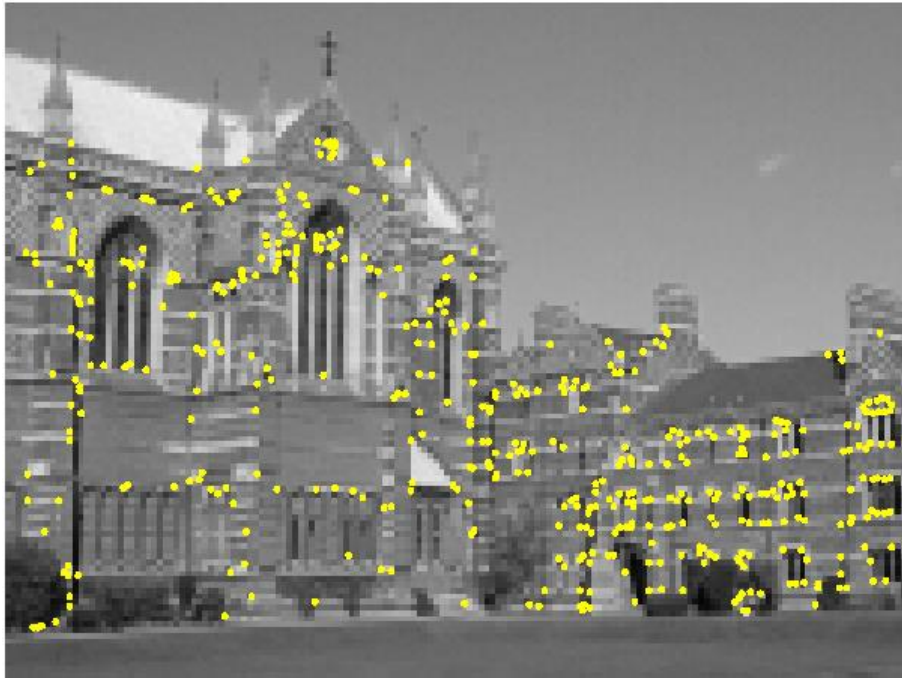
Detected Corners
