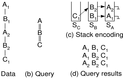
Figure 3: Compact encoding of answers using stacks.
