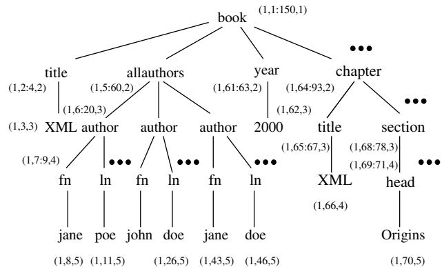
Figure 1: A sample XML Tree representation
