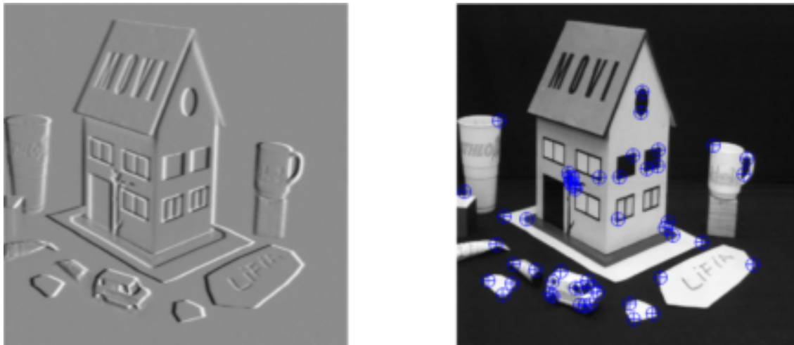
Figure 2: x-component of the gradient I_x (left) and the top 50 detected corner points (right) on the image house.pgm , both with \sigma = 1 . Your report should also include the y-component of the gradient I_y and results for different values of \sigma on the desk images.
