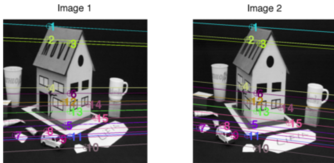
Figure 1: 15 hand-clicked points on the stereo pair house1.gif and house2.gif were used to compute the fundamental matrix F . Plot shows the locations of these 15 points in both images and their corresponding epipolar lines.
