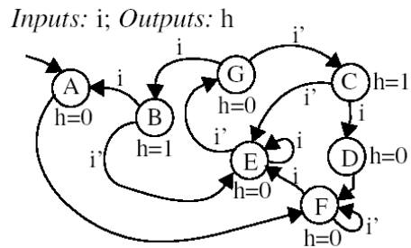
Figure 6.92: FSM example.
