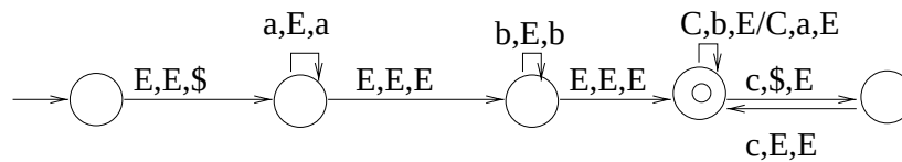
Fig. 1. Solution for 2.
