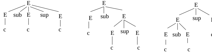
Fig. 2. Solution for 5.
