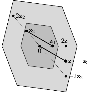
Figure 5. Minkowski's theorem
