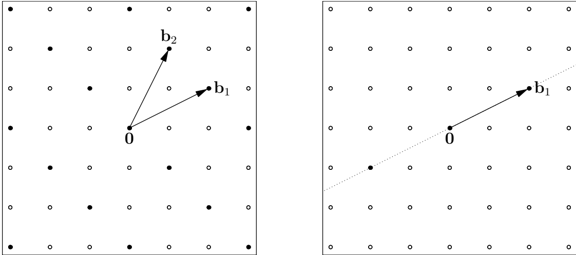
Figure 2. Two sublattices of \mathbb{Z}^2 . \mathcal{L}(\mathbf{B}) , on the left, is a full rank sublattice because it is also 2-dimensional. \mathcal{L}(\mathbf{b}_1) on the right is a full sublattice of \mathbb{Z}^2 because it contains all lattice points in its linear span. On the other hand \mathcal{L}(\mathbf{B}) is not a full sublattice of \mathbb{Z}^2 .
