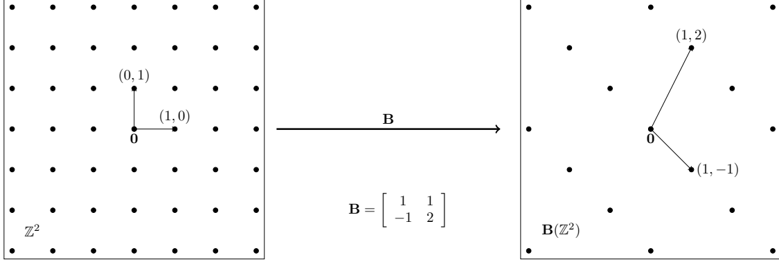
Figure 1. The integer lattice \mathbb{Z}^2 , and the two dimensional lattice \mathcal{L}(\mathbf{B}) = \mathbf{B}(\mathbb{Z}^2) generated by the basis vectors \mathbf{b}_1 = (1, -1) and \mathbf{b}_2 = (1, 2) . The lattice \mathcal{L}(\mathbf{B}) is the set of all integer linear combinations of the basis vectors, and can alternatively be described as the result of applying a linear transformation \mathbf{B} to the integer lattice \mathbb{Z}^2 .
