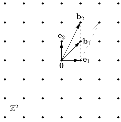
Figure 3. [e_1, e_2] and [b_1, b_2] are two different bases for the integer lattice \mathbb{Z}^2 . Clearly, \mathcal{L}([b_1, b_2]) \subseteq \mathbb{Z}^2 because b_1, b_2 are integer vectors. We also have \mathbb{Z}^2 \subseteq \mathcal{L}([b_1, b_2]) because both unit vectors e_1, e_2 can be expressed as integer linear combinations of b_1, b_2 .
