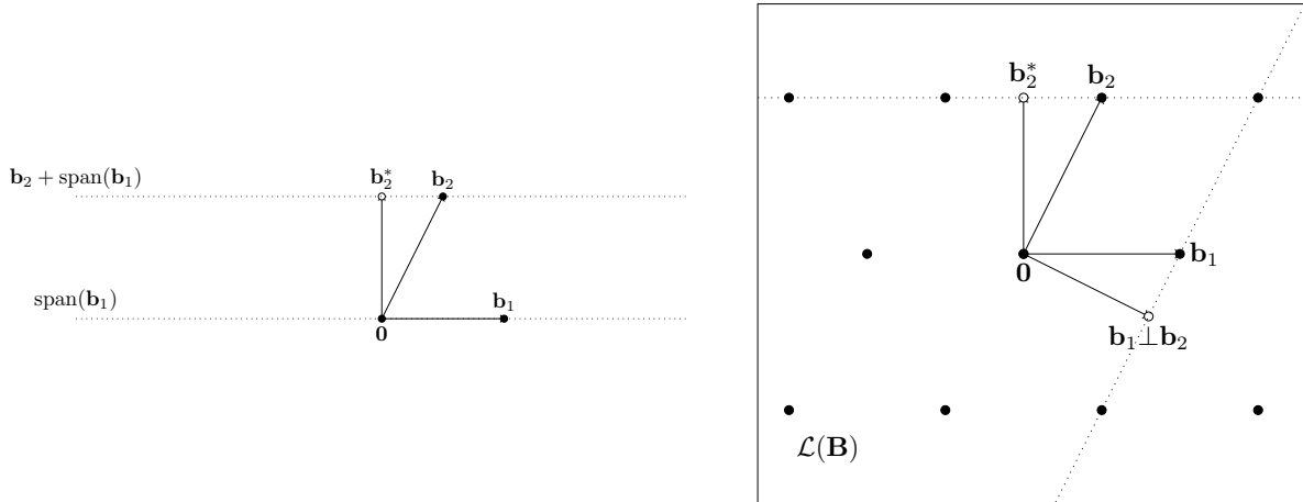
Figure 4. A basis \mathbf{b}_1, \mathbf{b}_2 and its Gram-Schmidt orthogonalization \mathbf{b}_1^*=\mathbf{b}_1, \mathbf{b}_2^* . The orthogonalized basis depends on the order of the basis vectors: the basis \mathbf{b}_2, \mathbf{b}_1 has orthogonalization \mathbf{b}_2^*=\mathbf{b}_2, \mathbf{b}_1^*=\mathbf{b}_1 \perp \mathbf{b}_2
