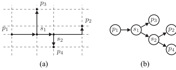
Fig. 2. 4-pin net example of a Steiner tree and its corresponding RC tree constructed for net delay calculation. (a) Steiner tree example. (b) Corresponding RC tree.
