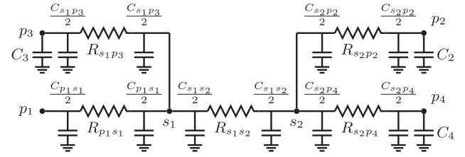
Fig. 3. Elmore delay model for the above 4-pin net example.
