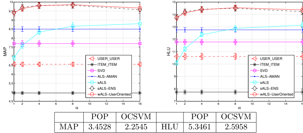
(a) Yahoo news data
