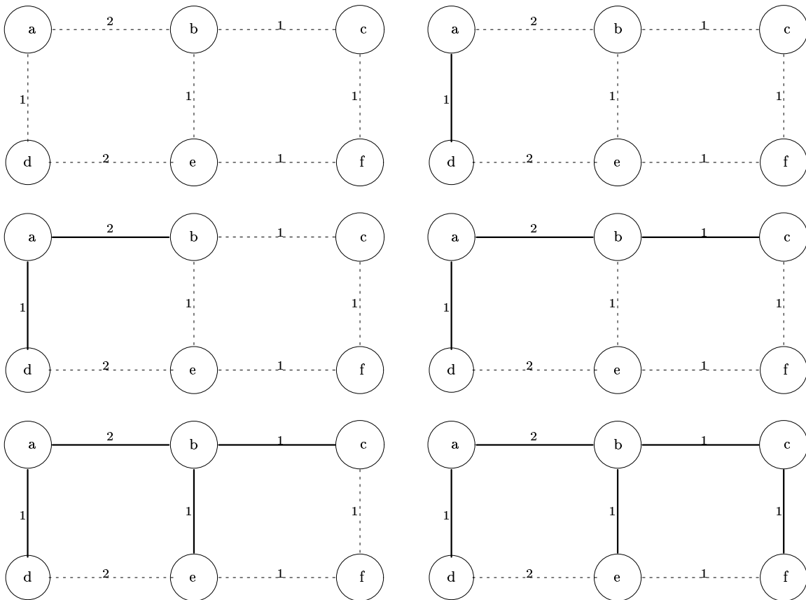
Figure 1: The progression of Dijkstra's algorithm for part a. Note: This is not the only correct solution
