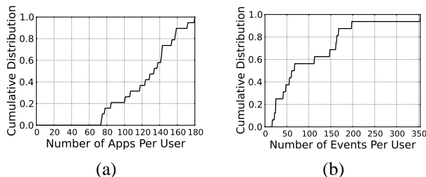
Figure 7: Distribution of the number of apps and events.
