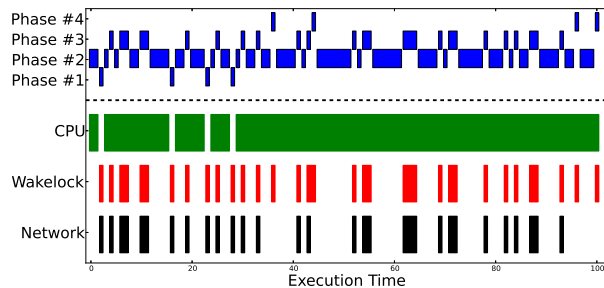
(a) Phase pattern based on RTV
