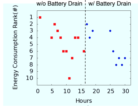
Figure 2: Battery consumption rank of the Android Gallery app running on a real user’s phone. We recorded the battery consumption rank of this app reported by the Android “Battery Usage” utility, once every hour. The first 15 hours is the time period when the app does not have the battery bug, whereas the second 15 hours is the period when the bug manifested.
