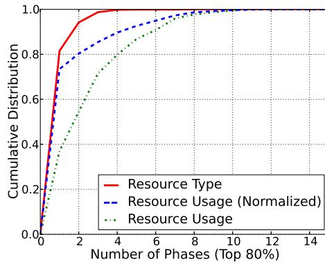
Figure 8: The cumulative distribution of number of phases across 1,890 apps we monitored on real user phones during the user study. We only consider the major phases that account for 80% of the total execution time.
