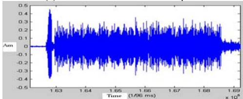
(b) OFDM waveform received
