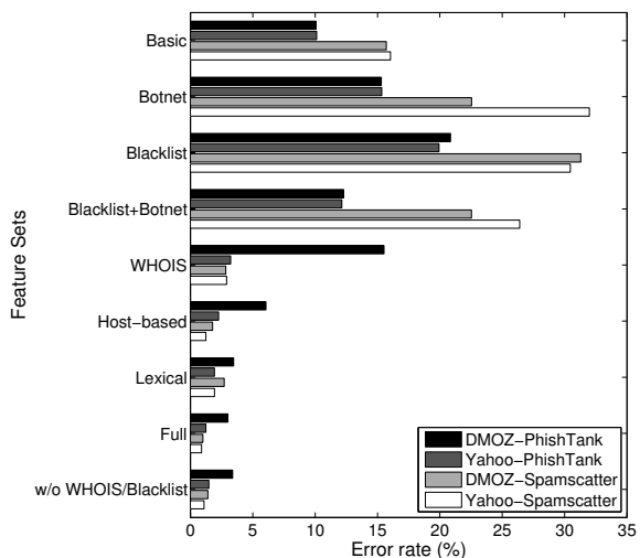
Figure 1: Error rates for LR with nine feature sets on each of the four URL data sets. Overall, using more features improves classification accuracy.
