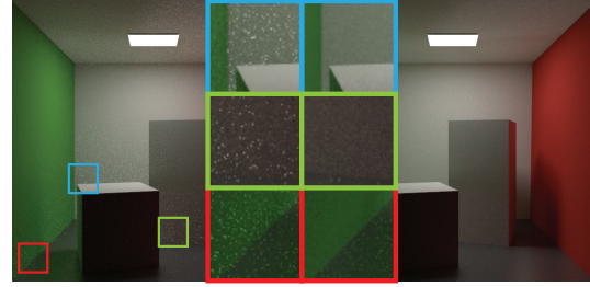
Figure 8: Evaluation of MIS upper bound weights. Left: results with standard MIS weights; Right: same scene computed with our upper bound MIS weights for correlated paths as proposed in Sect. 5. Noise is reduced significantly with our improved weights.
