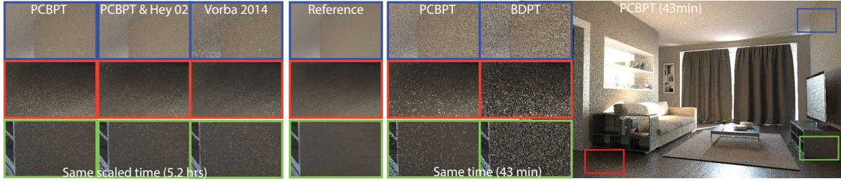
Figure 11: Same time comparisons for Living Room scene. Inset results left to right: PCBPT (78k iterations), PCBPT combined with [Hey and Purgathofer 2002] (2241 iters), [Vorba et al. 2014] for 5.2 hours of computation (wall-clock (unscaled) time for [Vorba et al. 2014] 1h); reference; PCBPT, BDPT after 43 minutes and 1100 iterations. Right: PCBPT image.
