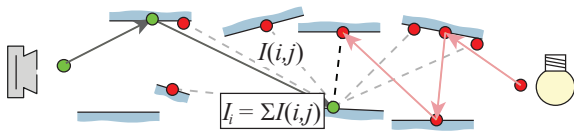
Figure 6: The contribution of a single connection is I(i, j) for strategy i (i.e., eye sub-path lengths of i = 3 here) and light sub-path j (red). I_i is the sum of all such contributions, which we estimate probabilistically.
