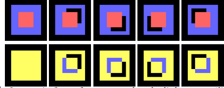
Figure 4: Images in figure 3 are warped to the light center (line 5 precomputation pseudocode). On top, we show the first layer after warping, and below, the second layer. Yellow indicates absence of a second layer i.e. only one layer present. Regions not visible from a given light position show up as holes (black) when warped.
