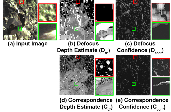
Figure 6. Verifying Depth Estimation and Confidence. The red patch refers to a region with repeating patterns. Defocus performs better in showing the region is farther away from the camera (b) with higher confidence (c). Correspondence shows unstable results (d) with lower confidence (e). The green patch refers to a region with bright and dark regions. Defocus gives incorrect depth values (b) with lower confidence (c). Correspondence gives better results (d) with higher confidence at feature edges (e).
