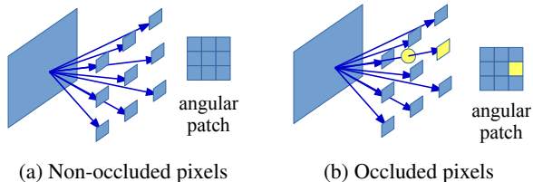
Figure 2: Non-occluded vs. occluded pixels. (a) At non-occluded pixels, all view rays converge to the same point in the scene if refocused to the correct depth. (b) However, photo-consistency fails to hold at occluded pixels, where some view rays will hit the occluder.
