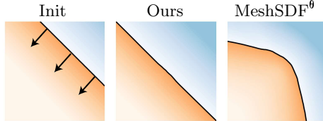
Fig. 3: MeshSDF \theta does not follow the level-set equation. (Left) A planar surface defined implicitly with an MLP is influenced by a flow field in the direction of its normal. The motion attained using differentiable iso-surface extraction (Right) is inconsistent with the field. Our method (Center) propagates the front as expected.
