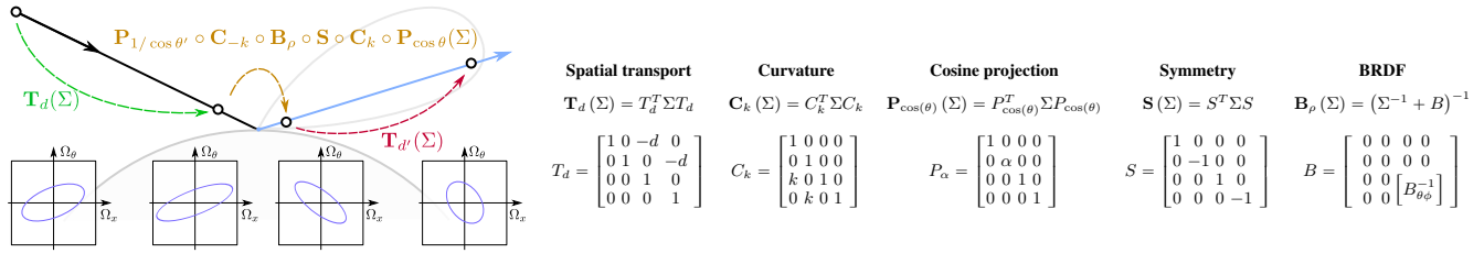
Fig. 4. Covariance tracing [Belcour 2012] predicts the matrix of second moments, \Sigma , of the light field spectrum (depicted as ellipsoids, bottom left insets). \Sigma is predicted for a given light path by composing individual matrix operators (top left). These operators have simple analytic forms, as depicted in the right of the Figure: free-space transport and object curvature operators are shears in covariance-space, while the BRDF reflection operator acts as an angular bandlimiting kernel. We introduce a more efficient evaluation of the BRDF matrix operator in Appendix A.
