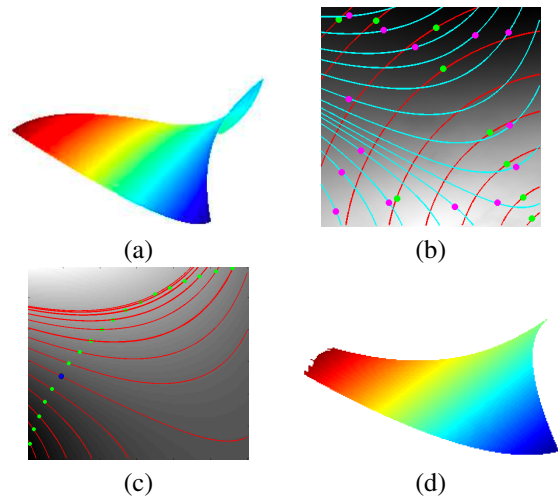
Fig. 9. Depth recovery for a monkey saddle surface. (a) The ground truth surface. (b) Recovered isocontours of constant \|\nabla z\| (red) and constant z (cyan), from images under a Torrance-Sparrow BRDF model. All points on the red and cyan curves have same depths as the respective green and magenta points. (c) Specifying the surface normal at one point (marked in blue) on the surface determines all depths along the corresponding isocontour of constant \|\nabla z\| (green points), from which depth at every other point can be determined by tracing isocontours of constant z (red curves). (d) The reconstructed surface by tracing all the isocontours.
