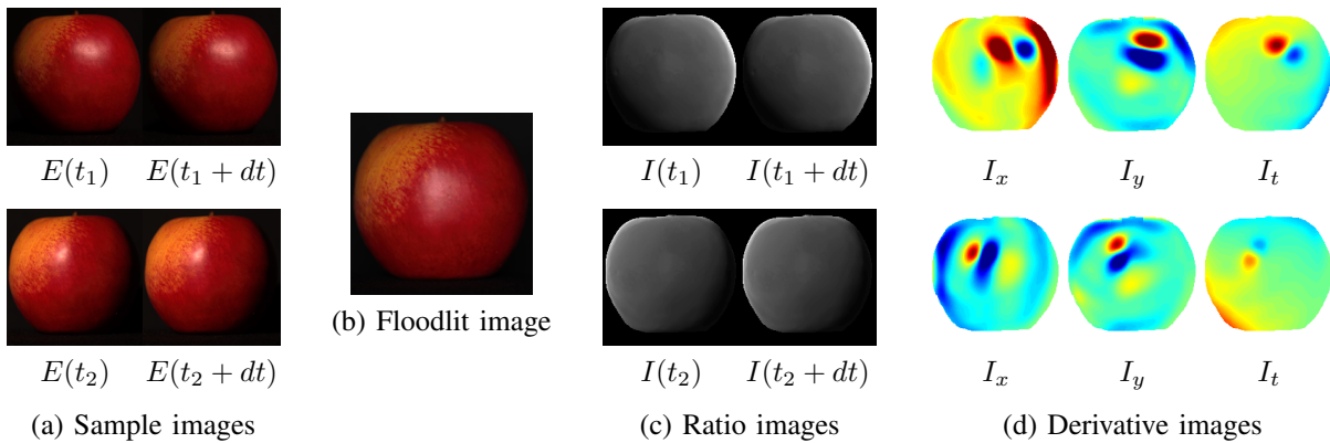
Fig. 12. Input pipeline for the apple dataset. (a) Sample images from the differential pair. (b) Floodlit image. (c) Ratios with respect to the floodlit image. (d) Spatial and temporal derivatives. Blue indicates low values and red indicates high values.
