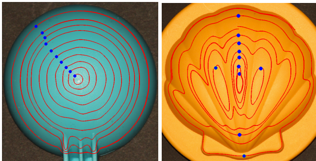
Fig. 4. Given a single real image of (a) a plastic spoon and (b) a plastic shell, the result of Proposition 1 is used to plot isocontours of constant \|\nabla z\| , shown in red, starting from the points marked in blue. No radiometric calibration of the input image is required.
