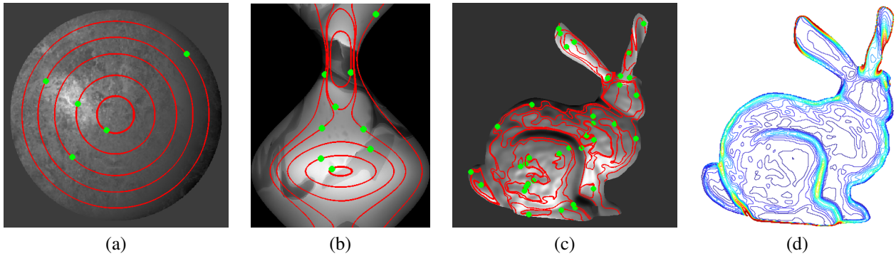
Fig. 6. Recovery of isocontours of constant \|\nabla z\| . Red curves plot the isocontours, while the green dots represent points chosen to start tracing the curves. (a) A sphere with variable albedo and simplified Torrance-Sparrow BRDF. (b) A vase with Blinn-Phong BRDF. (c) A bunny with Torrance-Sparrow BRDF. (d) Ground truth isocontours for the bunny.
