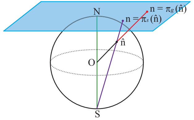
Fig. 2. An illustration of the two possible parameterizations for the surface normal. The gnomonic projection (red line) is denoted \mathbf{n} = \pi_g(\hat{\mathbf{n}}) and the stereographic projection (purple line) is denoted \mathbf{n} = \pi_s(\hat{\mathbf{n}}) .
