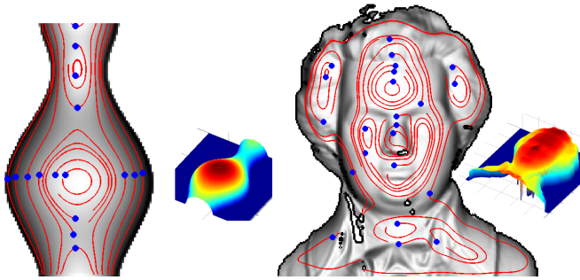
Fig. 3. Illustration of Proposition 1 on synthetic data corresponding to (a) a vase and (b) a Mozart figurine. Given a single image from a sensor collocated with a light source, isocontours of constant \|\nabla z\| are computed. All points on the red curves have the same depth as the corresponding blue dot. The ground truth depth map is shown for reference in the inset.
