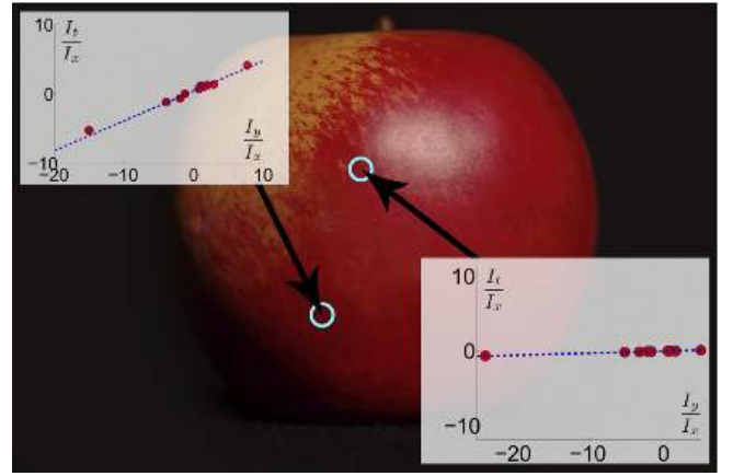
Fig. 5. The ratio of image derivatives at a pixel, recorded for various light positions, lie on a straight line given by the equation \lambda \frac{I_y}{I_x} + \kappa \frac{I_t}{I_x} = 1 .
