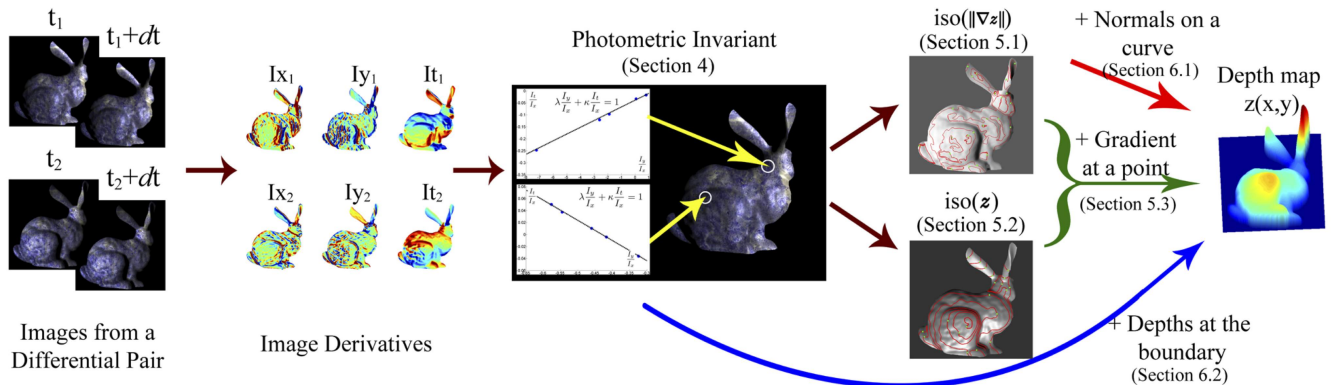
Fig. 1. An outline of our differential theory of photometric stereo. Two or more differential pairs lead to an uncalibrated photometric invariant. Isocontours of constant \|\nabla z\| and constant z may be recovered from the invariant. Additional information in the form of gradient at a single point suffices to recover depths. Normals on a curve or depths on the boundary can be used for a more noise robust estimation.
