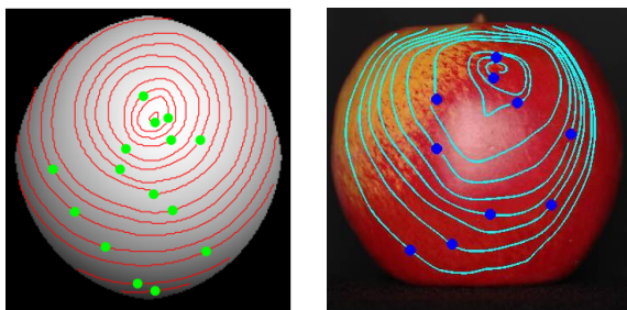
Fig. 11. Isocontours of constant \|\nabla z\| for real data corresponding to a hand-moulded clay ball and a plastic apple.
