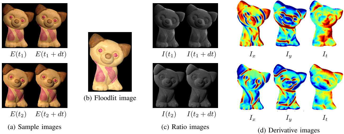
Fig. 15. Input pipeline for the toy dog dataset. (a) Sample images from the differential pair. (b) Floodlit image. (c) Ratios with respect to the floodlit image. (d) Spatial and temporal derivatives. Red stands for positive values and blue stands for negative values.
