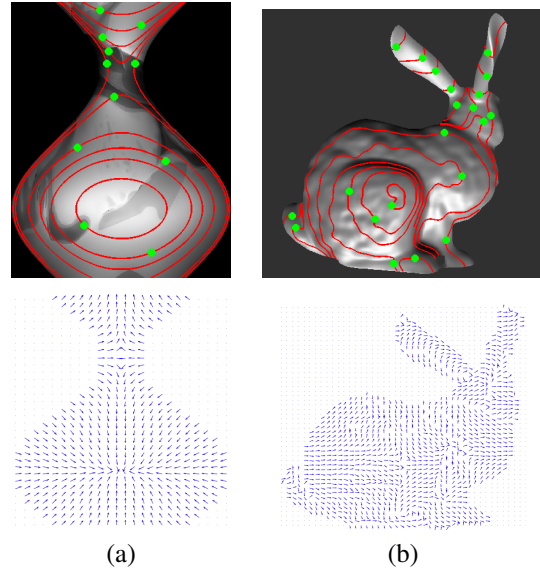
Fig. 7. Recovery of isocontours of constant depth. (Top row) Red curves plot the isocontours with the same depth as the green dots. (Bottom row) Plots of the direction of the gradient, with the length of the vector normalized to one for display. (a) A vase with variable albedo and Blinn-Phong BRDF. (b) A bunny with Torrance-Sparrow BRDF.
