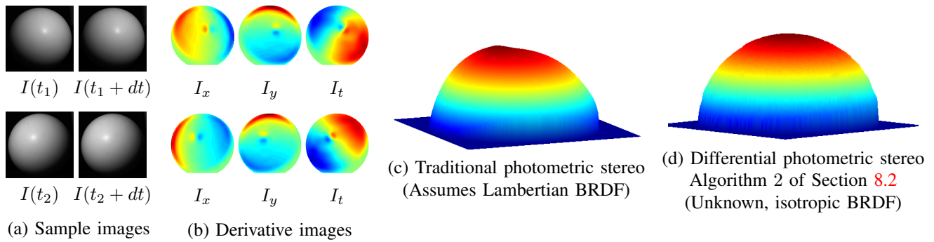
Fig. 14. Comparison with traditional Lambertian photometric stereo, using real data. (a) Two sample differential pairs of images of a teflon ball. (b) Spatial and temporal image derivatives. Red stands for positive values and blue stands for negative values. (c) Height recovered using traditional Lambertian photometric stereo. Note the shearing of the surface which is typically due to ignoring non-Lambertian effects. (d) Height recovered using the theory of Section 8.2.
