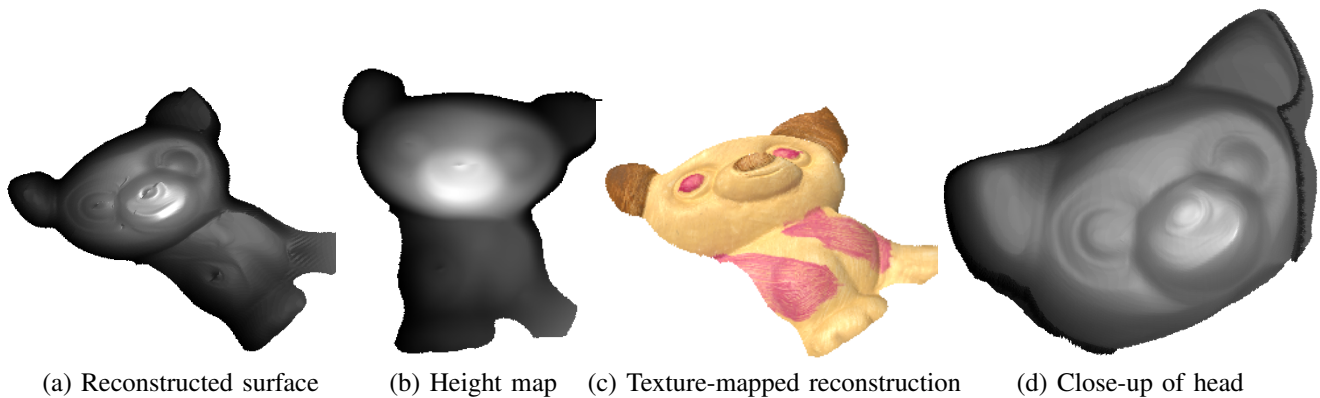
Fig. 16. Reconstruction for the toy dog using Algorithm 2 of Section 8.2, with Dirichlet boundary conditions. Note that the surface is not continuously differentiable, so does not strictly meet the requirements of our theory. Yet, the PDE solution is robust enough to recover a high quality depth map. (a) A top-and-side view of the recovered surface. (b) Recovered height map. Brighter shading indicates higher values. (c) A texture-mapped display of the 3D reconstruction. (d) A close-up reconstruction of the head.
