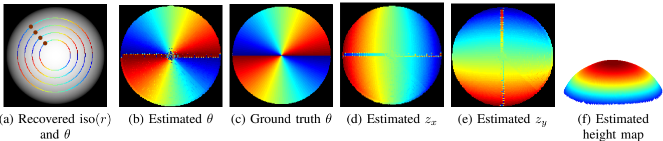
Fig. 10. Reconstruction for a synthetic sphere using Algorithm 1 of Section 8.1. (a) Isocontours of constant r = \|\nabla z\| computed using the estimated \lambda(x, y) , followed by estimation of \theta = \tan^{-1}\left(\frac{z_x}{z_y}\right) using seed values of the surface normal specified on the brown dots. The values of \theta are shown using a color-code that maps the interval \left[-\frac{\pi}{2}, \frac{\pi}{2}\right] between blue and red. (b) Recovered values of \theta , with the specified color map. (c) Ground truth \theta . (d) Estimated gradient in the x direction, z_x , red indicates large positive value and blue indicates large negative value. (e) Estimated gradient in the y direction, z_y , with the same color map. (f) Side view of the height recovered from integration of estimated z_x and z_y , which matches the ground truth shape. Red indicates higher heights and blue indicates lower heights.
