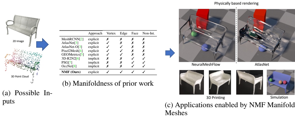
Figure 1: Given an input as either a 2D image or a 3D point cloud (a) Existing methods generate corresponding 3D mesh that fail one or more manifoldness conditions (b) yielding unsatisfactory results for various applications including physically based rendering (c). NeuralMeshFlow generates manifold meshes which can directly be used for high resolution rendering, physics simulations (see supplementary video) and be 3D printed without the need for any preprocessing or repair effort.
