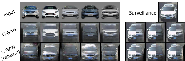
Figure 6: Web to SV (day) translation using CycleGAN (second) and its variant (third) by removing skip connection from generator and increasing receptive field size for patch discriminator. On the right, we overlay left half of translated images with SV image to highlight the impact of constraints on perspective transformation.
