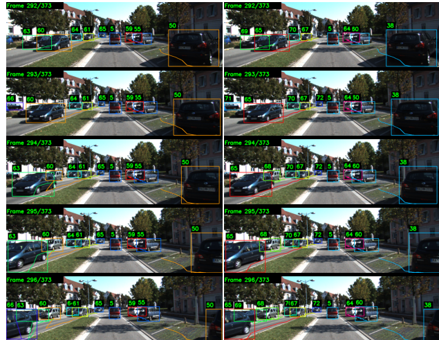
Figure 4: A qualitative example. Note the failure case of the model with hand-crafted costs (left) compared to the learned cost functions (right).
