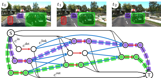
Figure 1: A network flow graph for tracking 3 frames [56]. Each pair of nodes corresponds to a detection. The different solid edges are explained in the text, the thick dashed lines illustrate the solution of the network flow.
