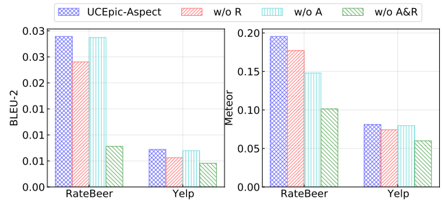
Figure 4: Ablation study on aspects and references.
