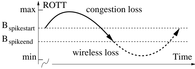
Fig. 3. Spike Scheme
