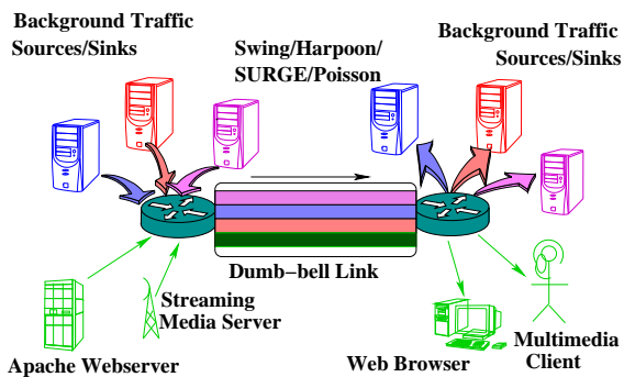
Figure 1: Evaluation architecture.
