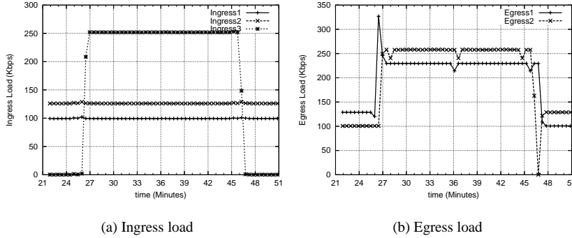
Figure 8: Functional evaluation.
