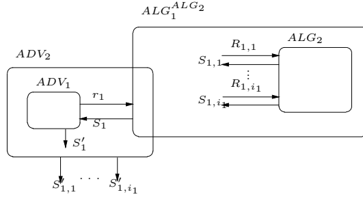
Fig. 1. One round of interaction between online algorithms for \Pi_1, \Pi_2 ALG_1, ALG_2 and the respective adversaries ADV_1, ADV_2 .
