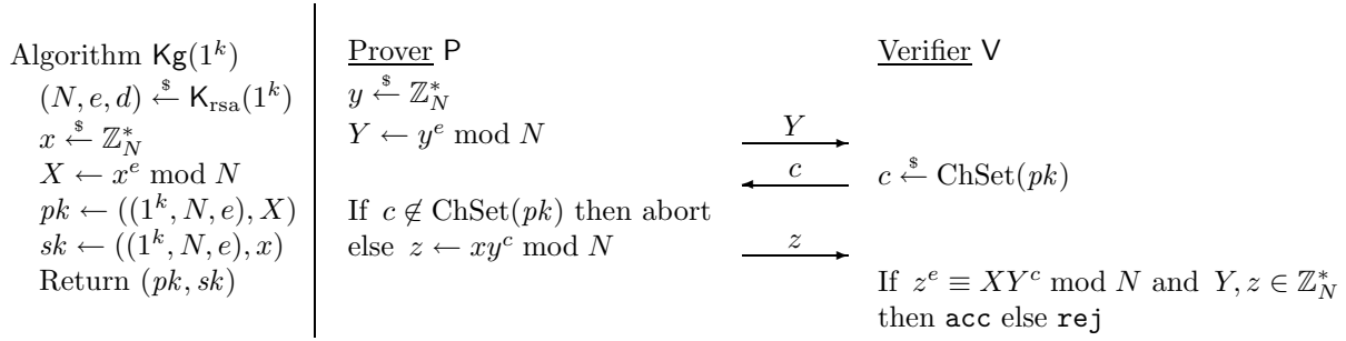
Figure 10: The \mathcal{S}\mathcal{H} -SI and \mathcal{S}\mathcal{H}^* -SI schemes. Both schemes are specified in terms of a prime-exponent RSA generator \text{K}_{\text{rsa}} and super-logarithmic challenge length l(\cdot) such that 2^{l(k)} < e for all (N, e, d) \in [\text{K}_{\text{rsa}}(1^k)] . The prover P and verifier V are initialized with states sk = ((1^k, N, e), x) and pk = ((1^k, N, e), X) , respectively. The \mathcal{S}\mathcal{H} -SI and \mathcal{S}\mathcal{H}^* -SI differ from each other in that the former uses challenge set \text{ChSet}(pk) = \{0, \dots, 2^{l(k)} - 1\} , while the latter uses \text{ChSet}(pk) = \{1, \dots, 2^{l(k)}\} .
