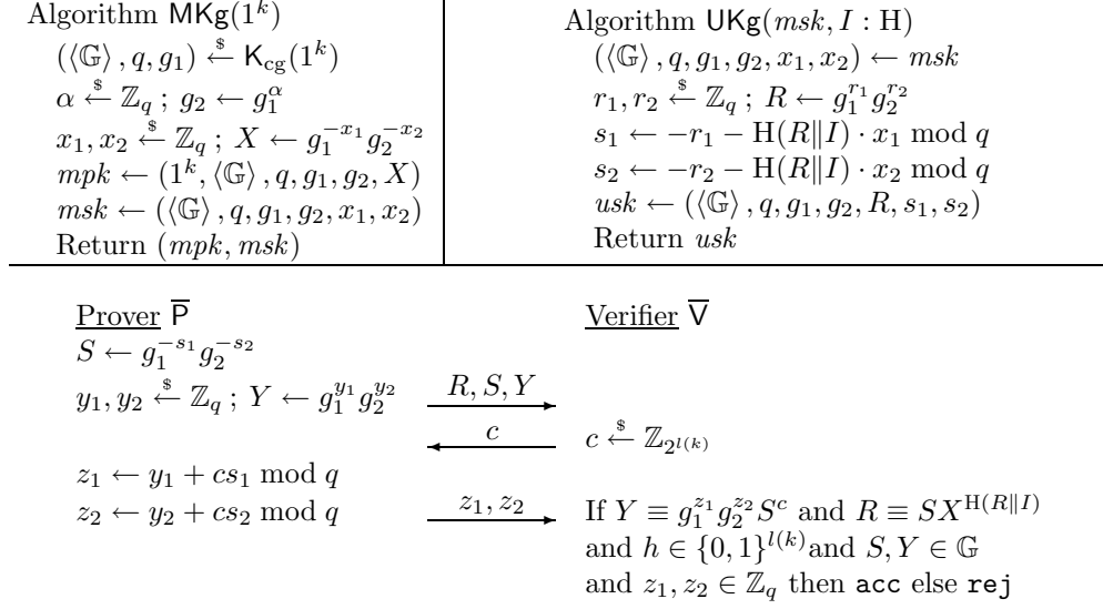
Figure 16: The OkDL-IBI scheme. The scheme is parameterized by super-logarithmic challenge length l : \mathbb{N} \rightarrow \mathbb{N} , a random oracle \text{H} : \{0, 1\}^* \rightarrow 0, 1^{l(k)} and a prime-order cyclic group generator \text{K}_{\text{cg}} such that 2^{l(k)} < q for all (\langle \mathbb{G} \rangle, q, g) \in [\text{K}_{\text{cg}}(1^k)] . The prover \bar{\text{P}} and verifier \bar{\text{V}} are run on initial states \text{usk} = (\langle \mathbb{G} \rangle, q, g_1, g_2, R, s_1, s_2) and (\text{mpk}, I) where \text{mpk} = (1^k, \langle \mathbb{G} \rangle, q, g_1, g_2, X) , respectively.
