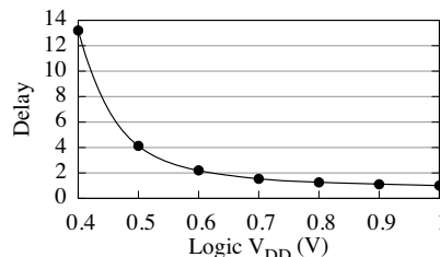
Figure 5: The Delay-Voltage curve for 28-nm logic.
