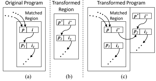
Figure 4. Example of CFG splicing
