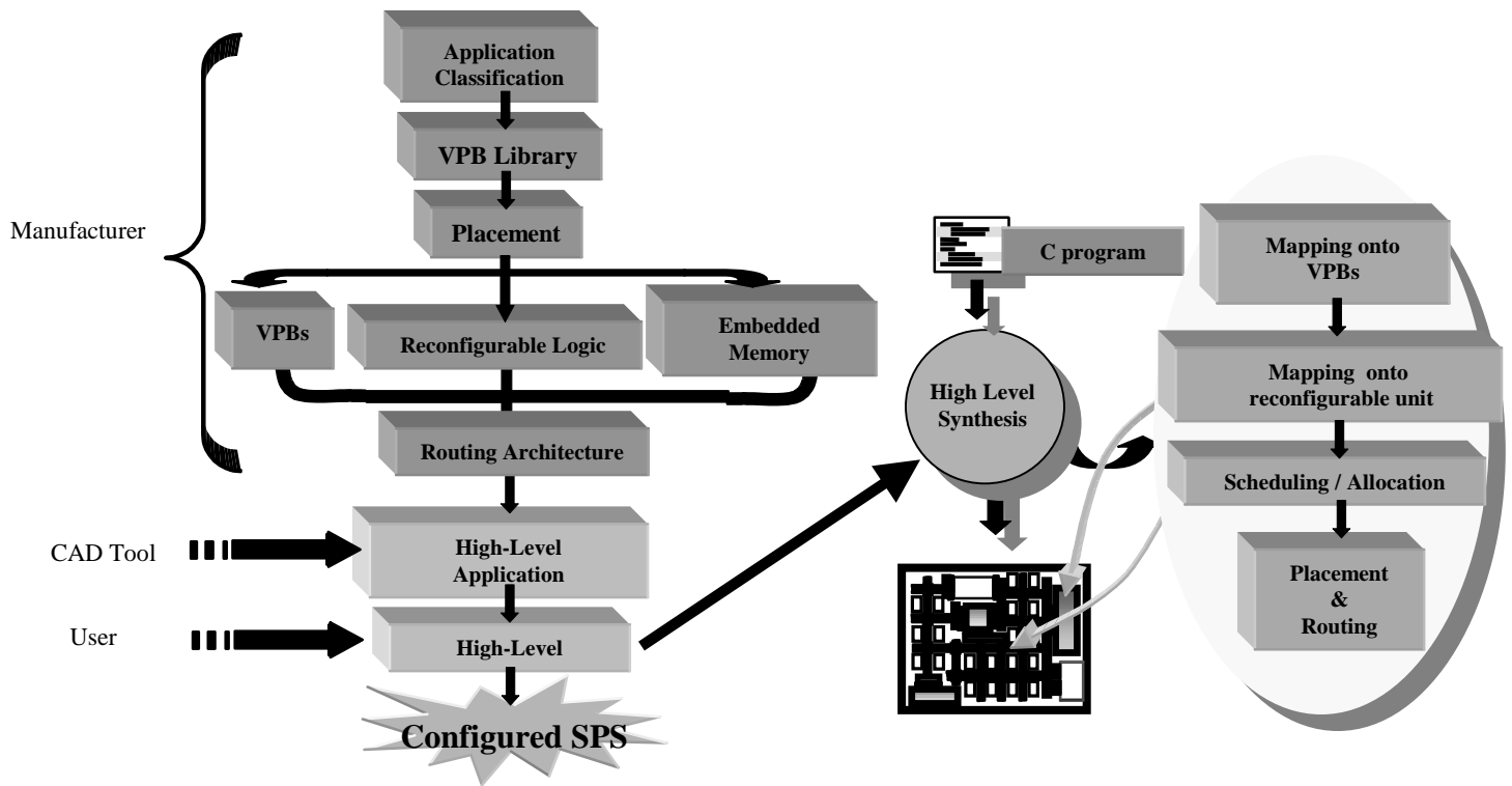
Figure 4.1 Strategically Programmable Systems Development and Implementation Flow
