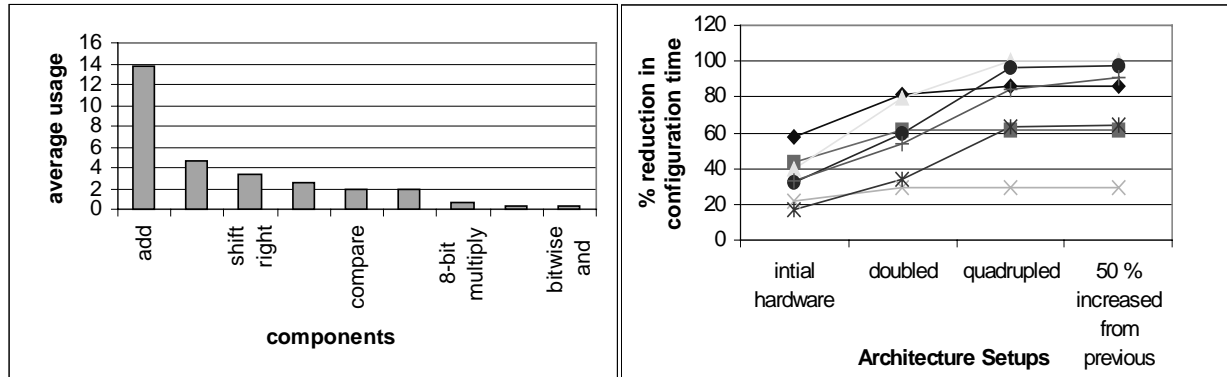
Figure 5.2.1a. Component utilization profile Figure 5.2.1b. Potential reduction in configuration time (each line representing a benchmark)
