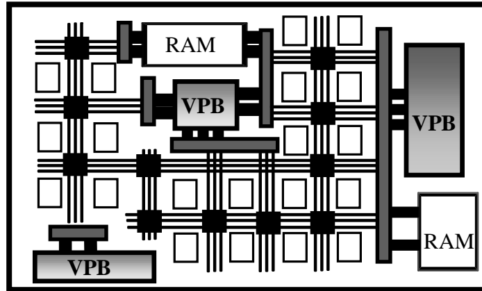
Figure 3.1.1 Sample SPS architecture
