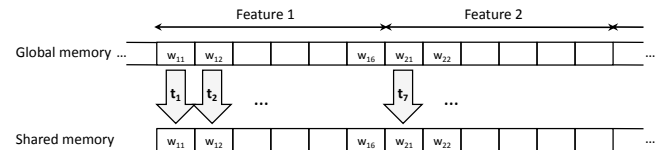
Figure 8. Threads t_1 \dots t_n loading features from global to shared memory.
