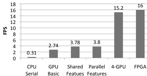
Figure 11. Performance of different implementations in FPS.
