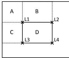
Figure 3. Method of calculating the value of a feature using the Integral Image.
