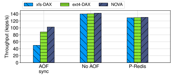
Figure 3. Redis MSET throughput. Making Redis’ core data structure persistent in NVMM (P-Redis) improves performance by 27% to 2.6 \times .
