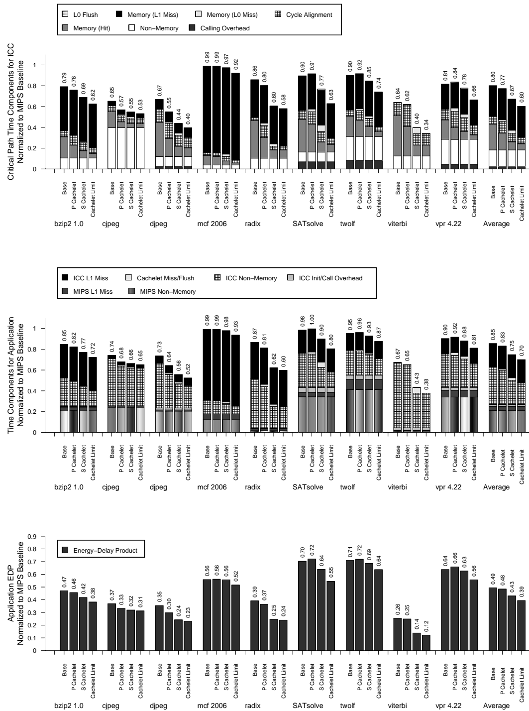
Figure 5.2: Cachelet performance and efficiency. The addition of cachelets greatly reduces latency and further improves EDP.
