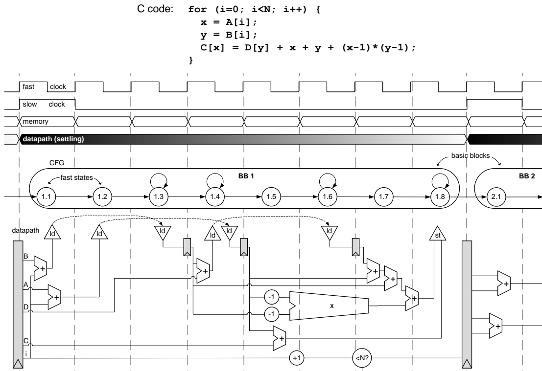
Figure 4.1: Example datapath and timing diagram demonstrating pipesplitting We show C source above a timing diagram, control flow graph, and datapath implementing that code. Under pipesplitting, non-memory datapath operators chain freely within a basic block, while memory operators and associated receive registers align to fast clock boundaries. The datapath contains arithmetic operators and load/store units for individual operations from the original program. The timing diagram shows how the datapath logic can take multiple fast cycles to settle while an ICC makes multiple memory requests.
