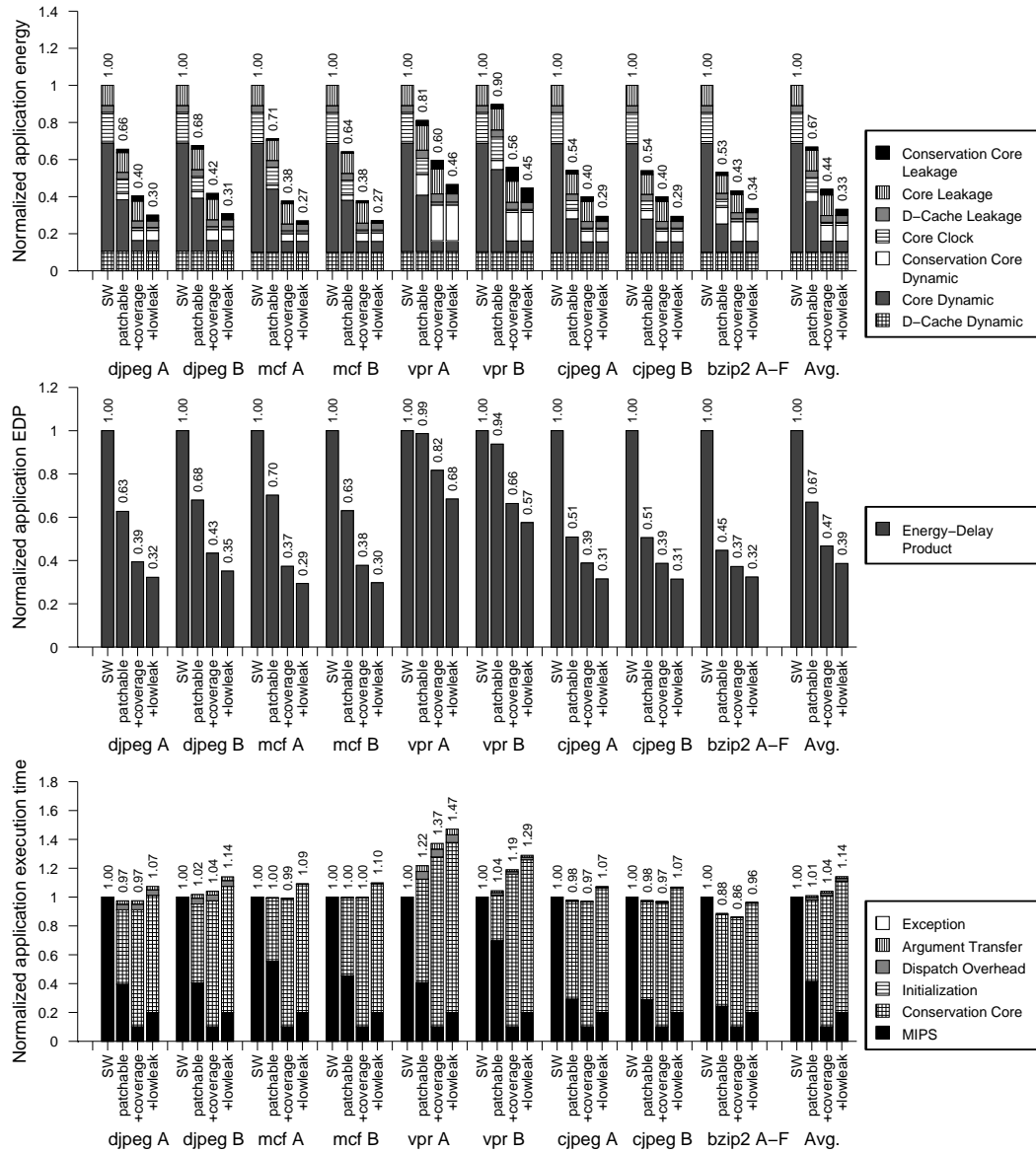
Figure 3.8: Full application system energy, EDP, and execution time for C-Cores, and projections for potential improvements These graphs show full application system energy, EDP, and execution time for C-Cores (lower is better). “SW” and “patchable” are as described in Figure 3.7. “+coverage” displays achievable improvements to energy reduction if 90% of the application can run in a C-Core. If a slower, lower-leakage process is used for the MIPS core in addition to improved coverage (“+lowleak”), even further improvements are possible. As in Figure 3.7, each subgroup of bars represents a specific version of an application, and for all six versions of bzip2 the C-Cores performance is identical.
