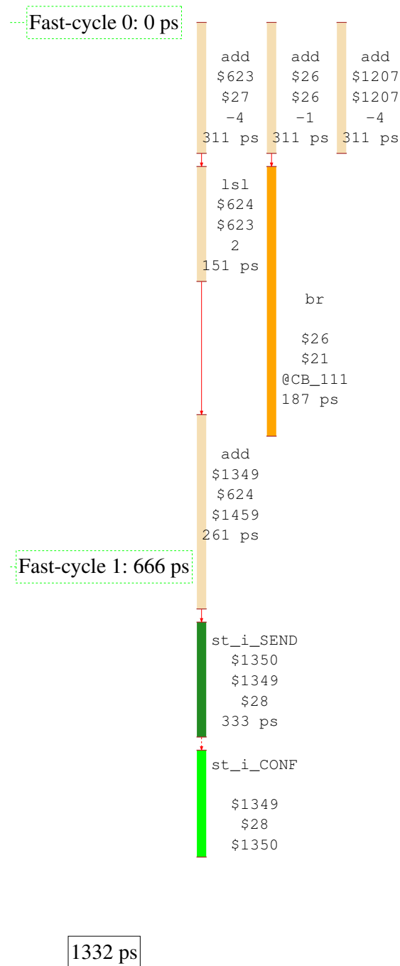
Figure 6.2: Schedule for a basic block with cachelets The addition of cachelets requires rescheduling under the assumption that cachelet accesses will be hits.
