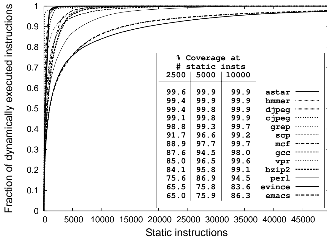
Figure 3.2: Dynamic coverage for given static instruction counts We show the cumulative distribution of dynamic coverage (on the vertical axis) as a function of the number of static instructions executed. For many x86 programs profiled, a small number of static instructions cover much of dynamic execution. This implies that a small amount of specialized hardware could cover large portions of execution for each of these programs.
