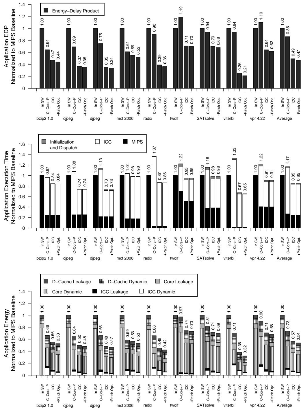
Figure 4.3: Application performance and efficiency with ICCs Application latency (middle), energy (bottom), and energy-delay (top) improvements from using ICCs can be large, with latency reductions of up to 35% and average EDP reductions of nearly 2x. The benefits of ICCs increase with application coverage.
