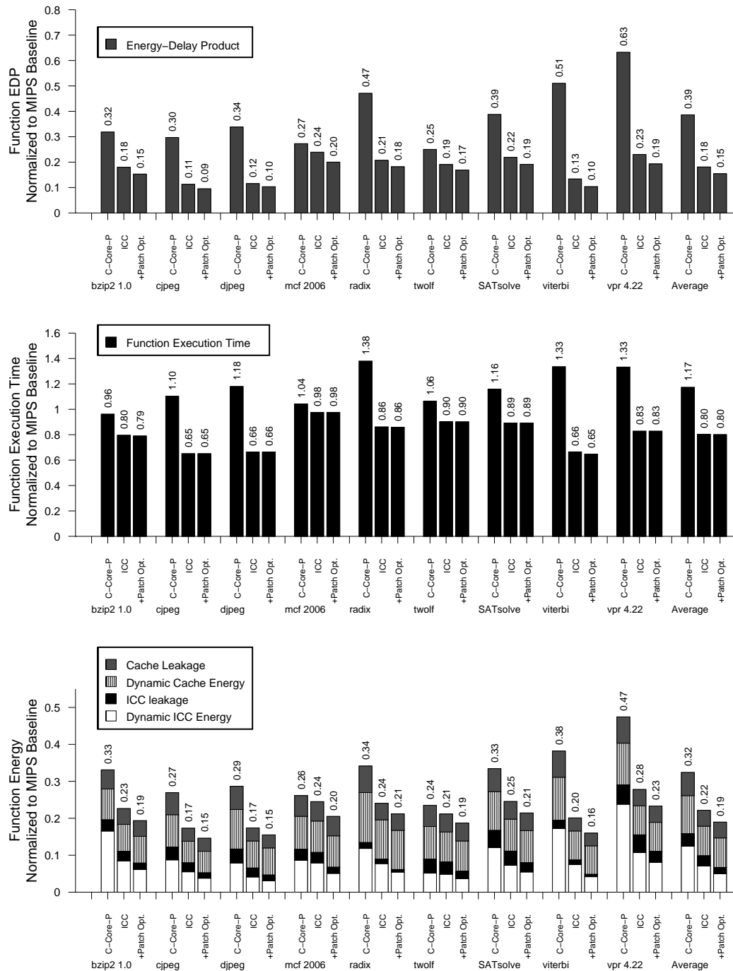
Figure 4.2: ICC performance and efficiency Pipesplitting allows the baseline ICC design to achieve lower latency (middle), and energy usage (bottom) compared to prototype C-Cores, resulting in significantly better energy-delay (top). Optimizing patching support decreases energy while maintaining performance and longevity.
