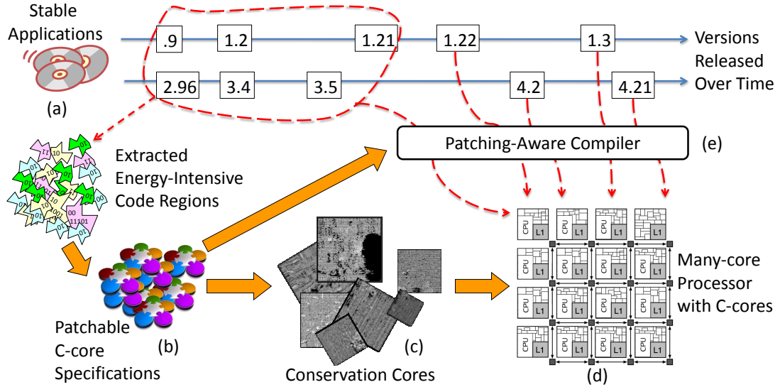
Figure 3.3: The C-Core Life Cycle A profiler (a) extracts a set of energy-intensive code regions from a corpus of stable applications in the processor’s target domain. The toolchain generalizes these regions into patchable C-Core specifications (b), translates them into circuits via an automated synthesis infrastructure (c), and integrates them into a multi-core processor (d). A patching-aware compiler maintains a database of C-Core specifications and generates binaries that execute on a combination of C-Cores and the local CPU. The compiler (e) generates a patching configuration that allows the C-Cores to run future (and past) versions of the original applications.
