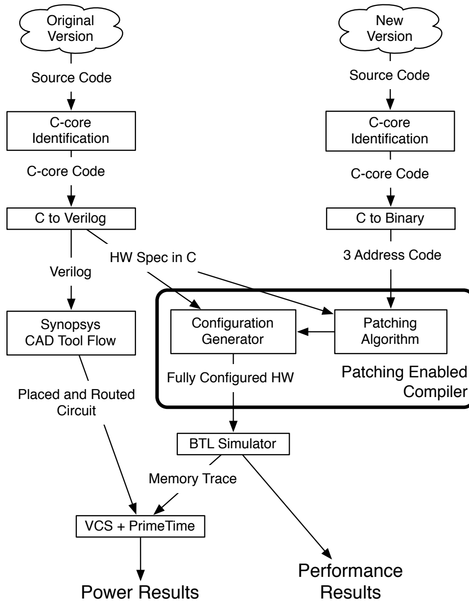
Figure 3.5: The C-Core C-to-hardware toolchain Our toolchain proceeds through hardware generation, patching, simulation, and power measurement over several stages. Program source enters our toolchain and passes through our C-Core selection stage, which identifies regions of code as C-Core candidates. Our C-to-Verilog compiler transforms these regions and produces a cycle-accurate simulator model for each region. Our simulator uses these models to produce traces, which we pass to VCS and PrimeTime to generate power results. The bold box contains the patch generation infrastructure based on our patching enabled compiler.
