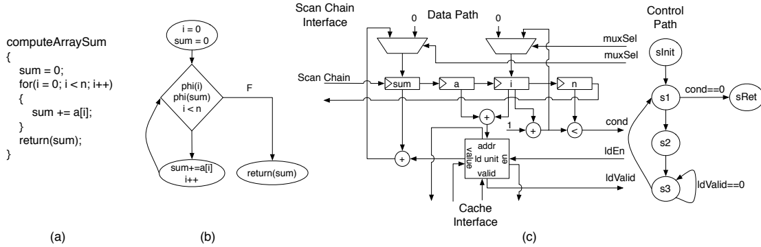
Figure 3.4: Conservation core example An example showing the translation from C code (a), to the compiler’s internal representation (b), and finally to hardware (c). The hardware schematic and state machine correspond very closely to the data and control flow graphs of the C code.
