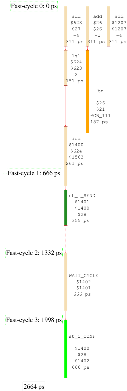
Figure 6.1: Schedule for a basic block Operations are shown annotated with estimated latency. Arcs are depicted showing the critical scheduling path for each operation.
