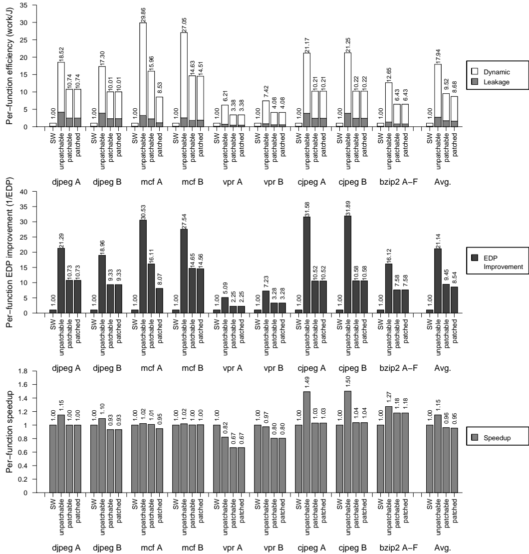
Figure 3.7: Conservation core energy efficiency Our patchable C-Cores provide up to 16\times improvement in energy efficiency compared to a general-purpose MIPS core for the portions of the programs that they implement. The gains are up to 2\times larger for non-patchable C-Cores, but their lack of flexibility limits their useful lifetime. Each subgroup of bars represents a specific version of an application (see Table 3.1). Results are normalized to running completely in software on an in-order, power-efficient MIPS core (“SW”). “unpatchable” denotes a C-Core built for that version of the application but without patching support, while “patchable” includes patching facilities. Finally, “patched” bars represent alternate versions of an application running on a patched C-Core. For all six versions of bzip2 (A-F), the C-Cores performance is identical.
