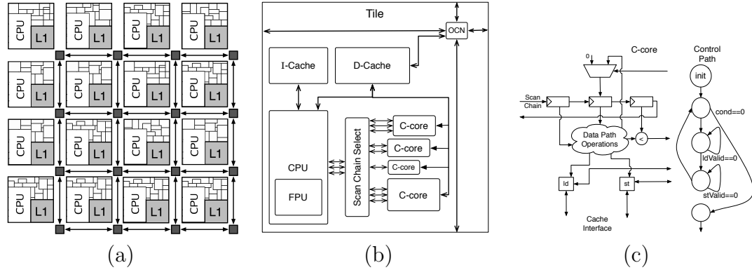
Figure 3.1: The high-level structure of a C-Core-enabled system A C-Core-enabled system (a) is made up of multiple individual tiles (b), each of which contains multiple C-Cores (c). Conservation cores communicate with the rest of the system through a coherent memory system and a simple scan-chain-based interface. Different tiles may contain different C-Cores. Not drawn to scale.
